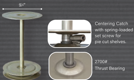
SIGNATURE HARDWARE DETAIL
